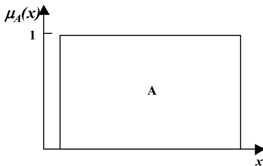
Fig. 7.9. Fuzziness of crisp set f(A) = 0 (minimum uncertainty).
