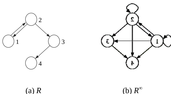
Fig. 3.10. Transitive closure
