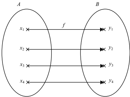
(c) Bijection
